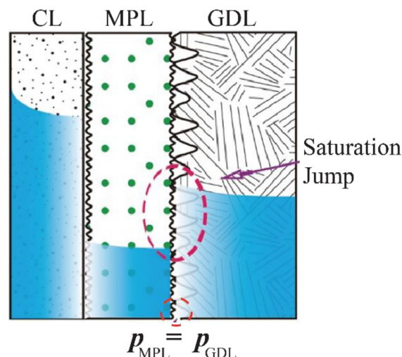
Fig. 15. Schematic diagram of liquid saturation jump at the interfaces between the catalyst layer (CL), microporous layer (MPL), and gas diffusion layer (GDL).
