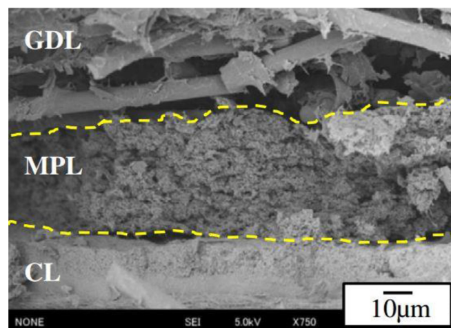
Fig. 16. SEM image of the through-plane cross section of the catalyst layer (CL), microporous layer (MPL), and gas diffusion layer (GDL) (reprinted from [66] with the permission of Elsevier).
