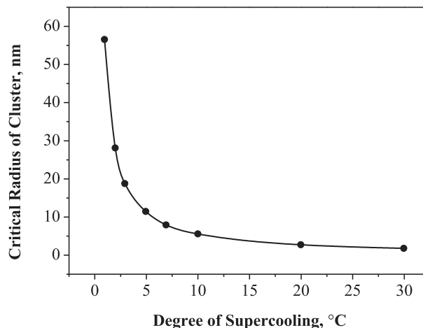
Fig. 13. Effect of temperature on critical cluster radius of supercooled water droplets (adapted from [98]).
