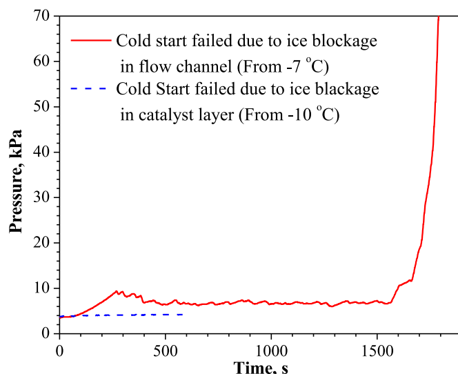
Fig. 18. Evolution of pressure drop in the cathode flow channel due to ice blockage (adapted from [25]).
